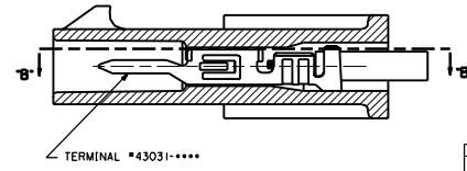
SECTION "D"-D" WITH TERMINAL SCALE: 8X1
