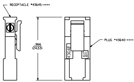
MATED MICRO-FIT CONNECTOR
