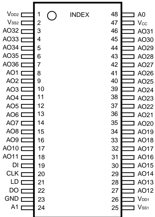
(DIP-48P-M01)
