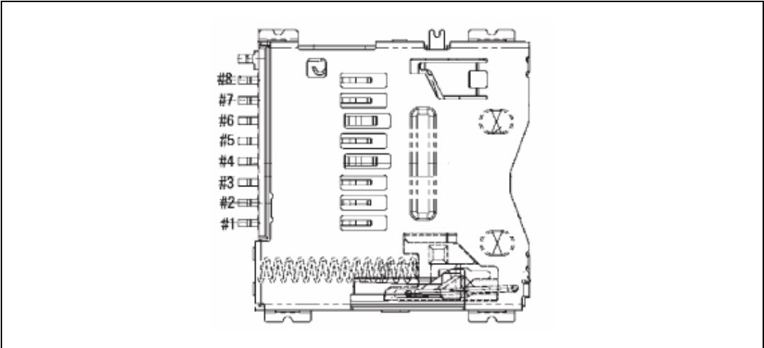
Figure 18. MicroSD connector CN15 (top view)
