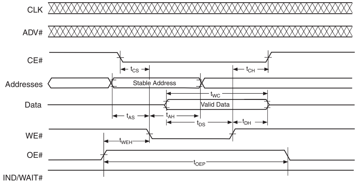
Figure I8.3 Asynchronous Command Write Timing
