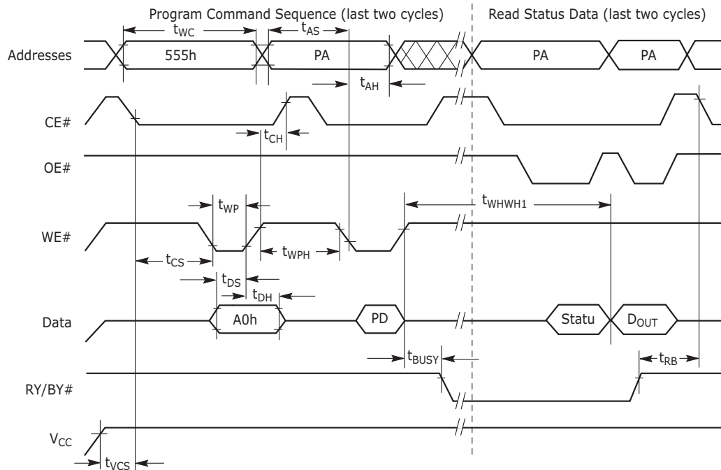
Figure 18.8 Program Operation Timings
