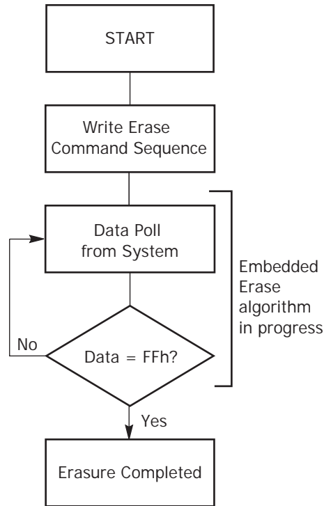
Figure 8.6 Erase Operation
