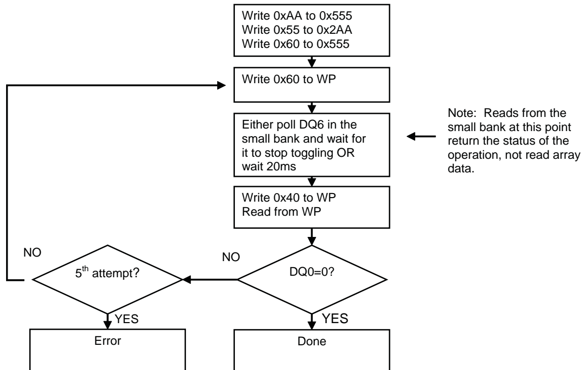
Figure 9.3 PPB Erase Operation
