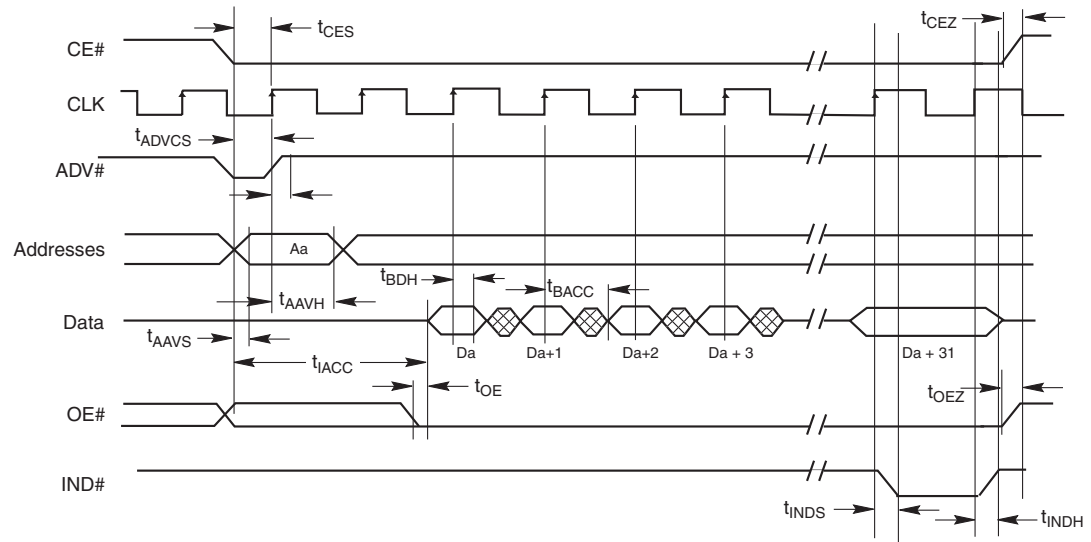
Figure I8.4 Burst Mode Read (x32 Mode)
