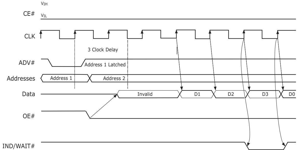
Figure 8.3 End of Burst Indicator (IND/WAIT#) Timing for Linear 8-Word Burst Operation
