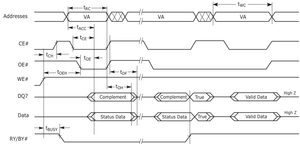
Figure I8.II Data# Polling Timings (During Embedded Algorithms)
