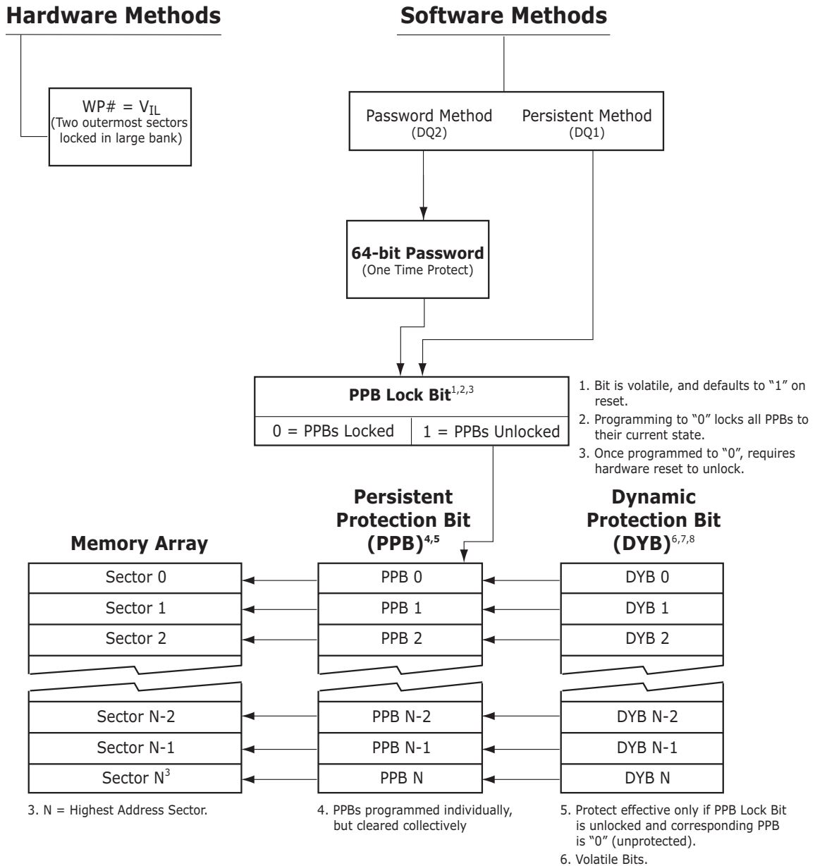
Figure 9.1 Advanced Sector Protection/Unprotection
