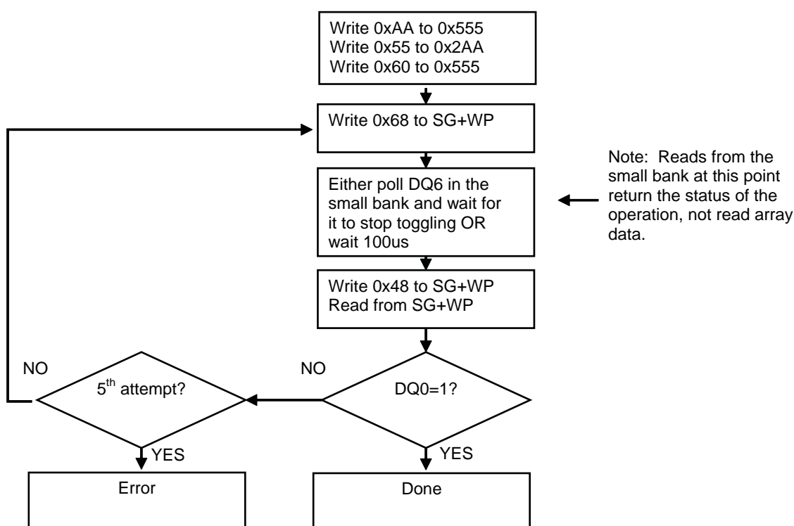
Figure 9.2 PPB Program Operation
