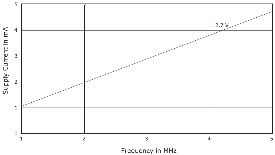
Figure 15.2 Typical I_{CCI} vs. Frequency
