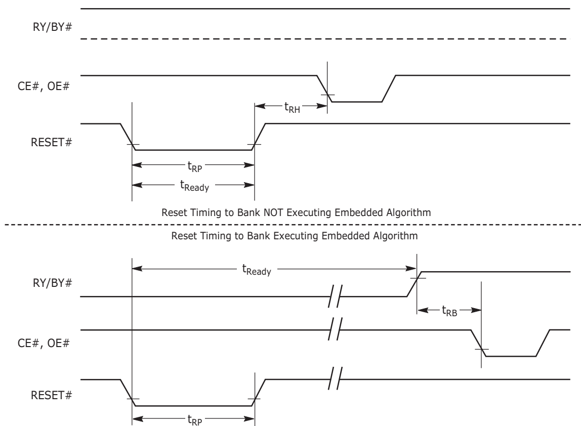
Figure I8.6 RESET# Timings
