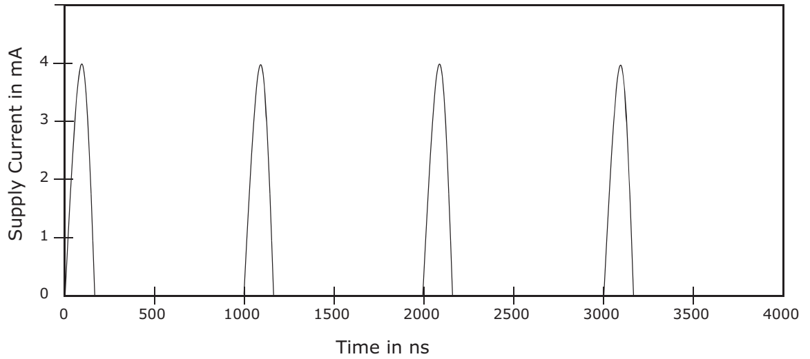
Figure 15.1 I_{CCI} Current vs. Time (Showing Active and Automatic Sleep Currents)
