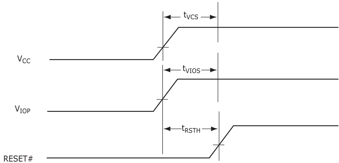
Figure I8.1 V_{CC} and V_{IO} Power-up Diagram
