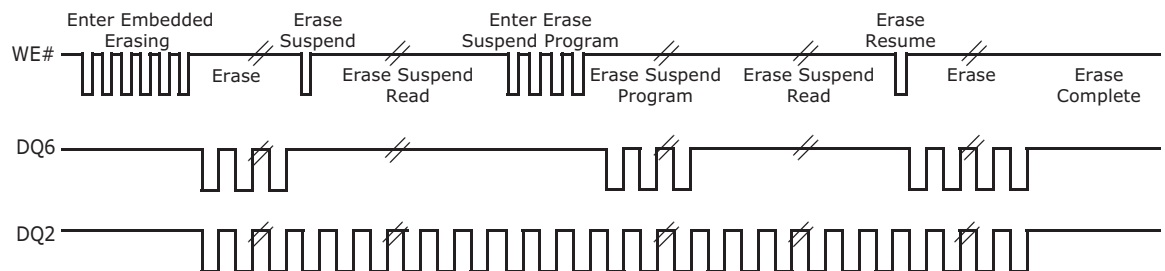
Figure I8.I2 Toggle Bit Timings (During Embedded Algorithms)
