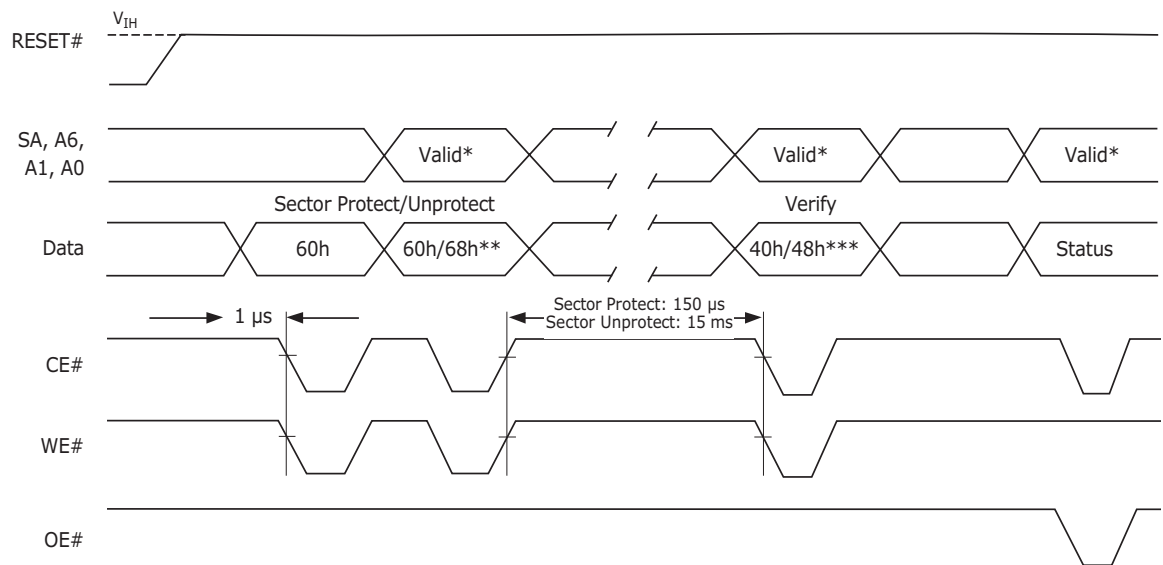
Figure 18.14 Synchronous Data Polling Timing/Toggle Bit Timings
