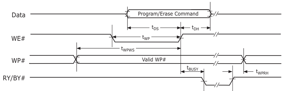
Figure 18.7 WP# Timing
