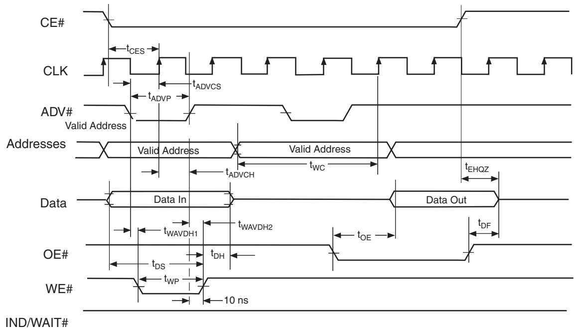
Figure I8.5 Synchronous Command Write/Read Timing
