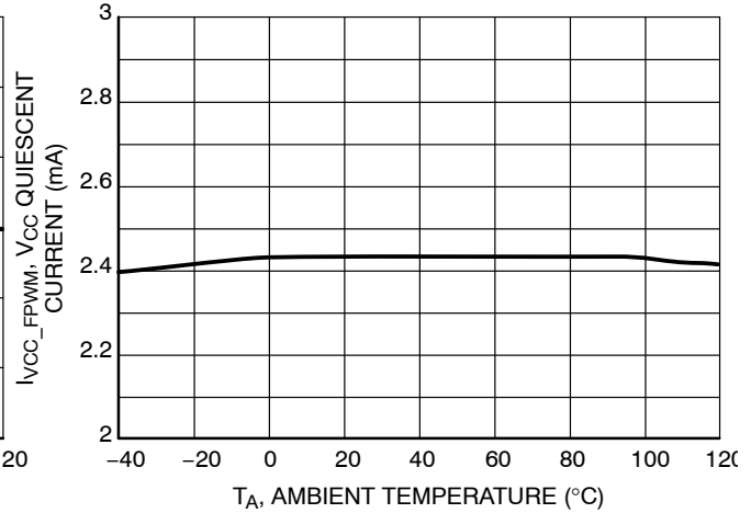
Figure 16. V_{CC} Quiescent Current vs. Ambient Temperature in FPWM Mode
