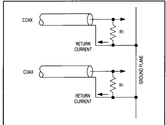
Figure 1. Low-Crosstalk Layout. Return current from the termination resistor does not flow through the ground plane.
