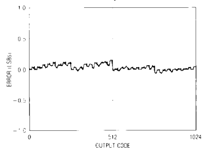
Linearity Plot
