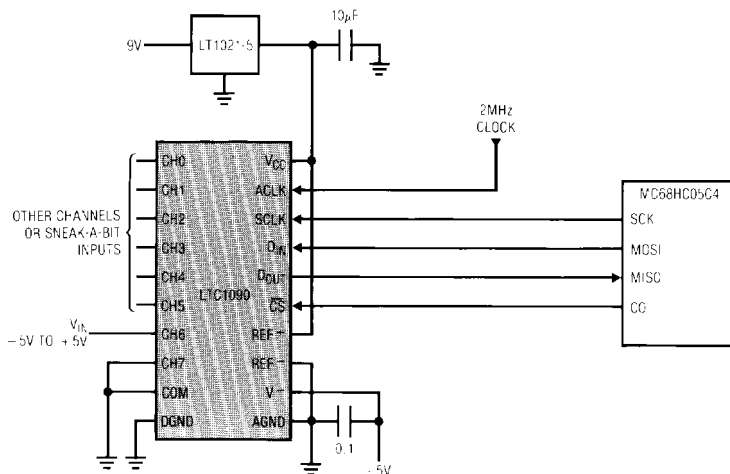
SNEAK-A-BIT Circuit
