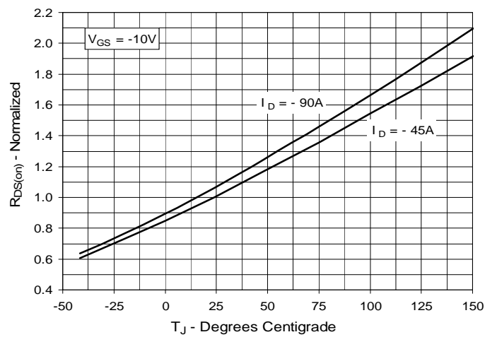
Fig. 4. R_{DS(on)} Normalized to I_D = -45A vs. Junction Temperature
