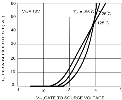
TRANSFER CHARACTERISTICS
