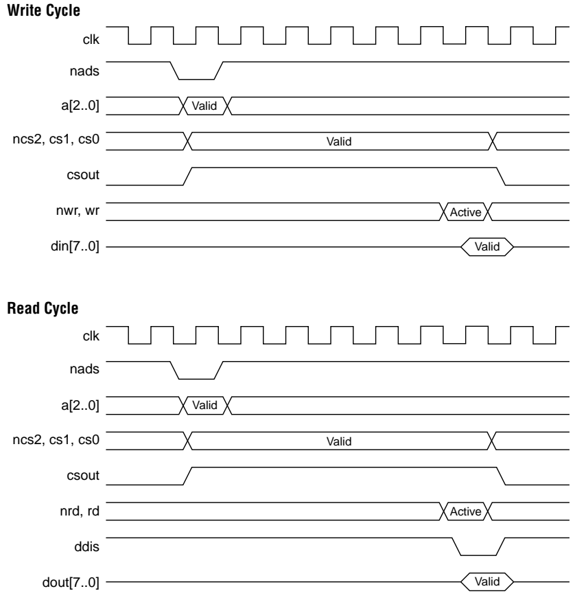
Figure 3. Read & Write Cycle Waveforms
