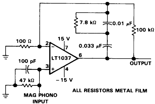
Figure 47. Phono Preamplifier
