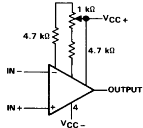
Figure 36. Improved Sensitivity Adjustment
