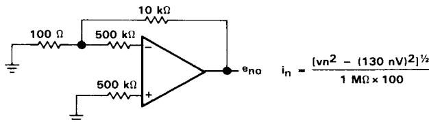
Figure 40. Noise Test Circuit
