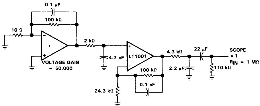
Figure 39. 0.1-Hz to 10-Hz Noise Test Circuit
