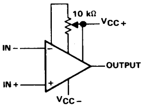
Figure 35. Standard Adjustment
