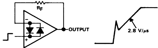
Figure 38. Pulse Operation
