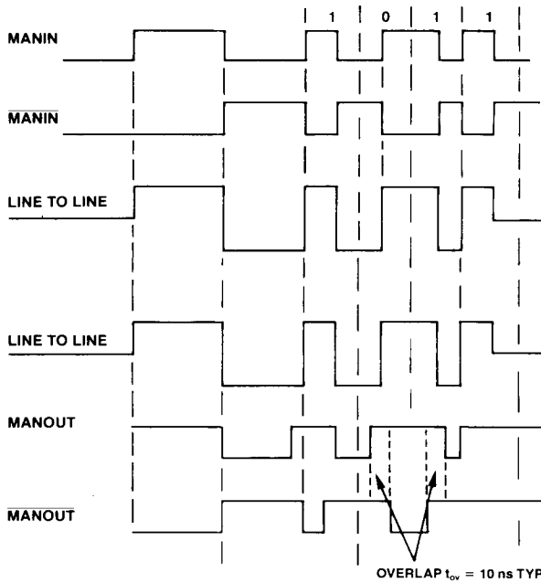
FIGURE 4: DRIVER LOGIC WAVEFORMS
