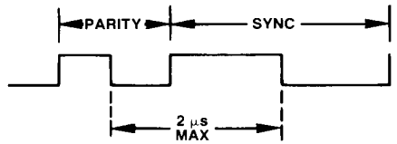
FIGURE 5: CONTIGUOUS WORD
