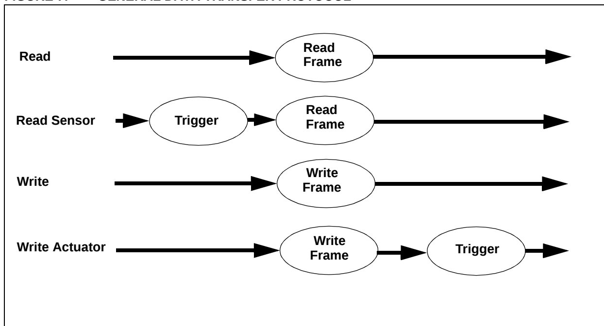
FIGURE 7: GENERAL DATA TRANSFER PROTOCOL
