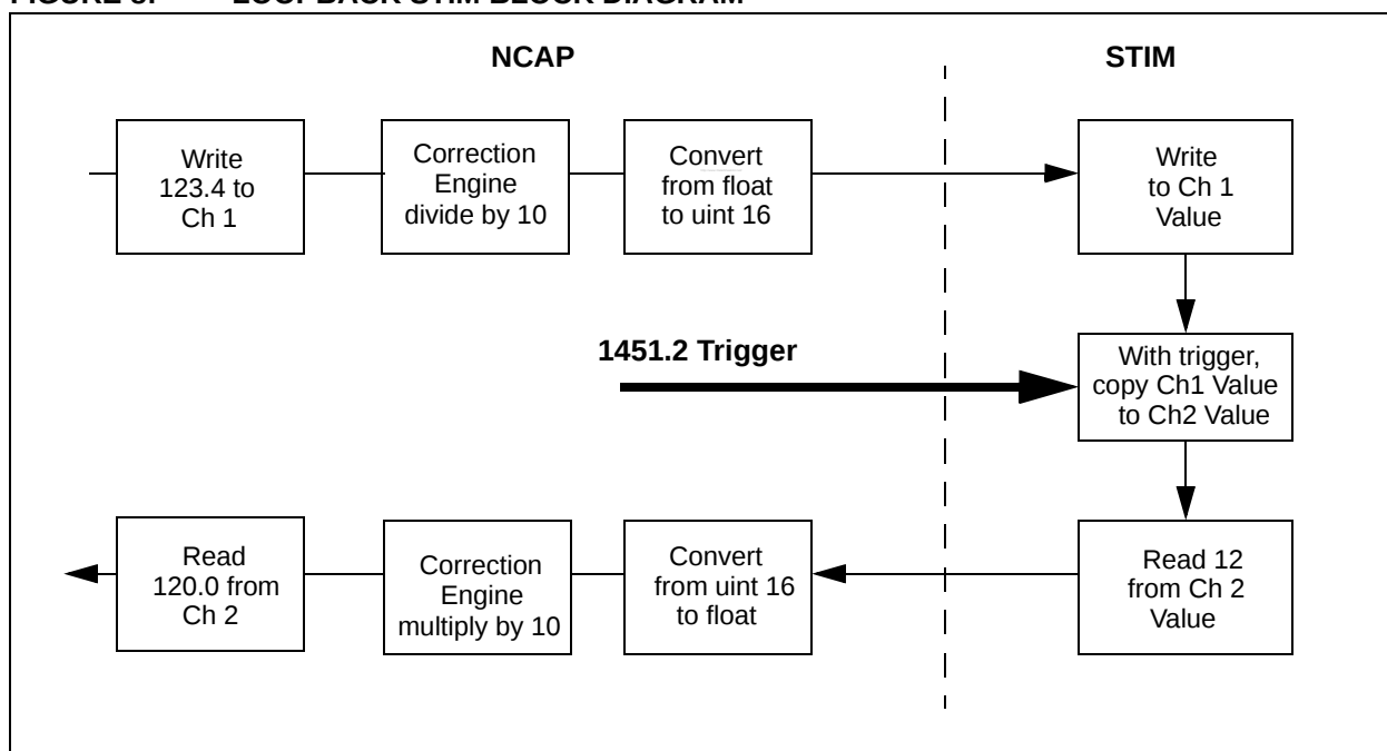
FIGURE 8: LOOPBACK STIM BLOCK DIAGRAM
