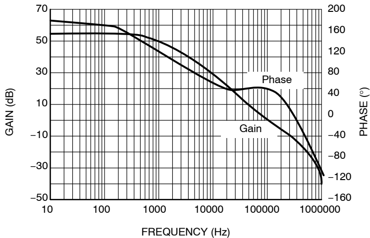
Figure 25. Phase and Gain Performance ( V_{IN} = 3.6\text{ V} , V_{OUT} = 1.2\text{ V} , I_{OUT} = 200\text{ mA} , Temperature = 25°C)
