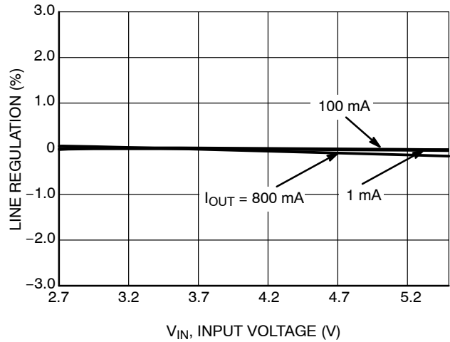
Figure 16. Line Regulation vs. Input Voltage ( V_{OUT} = 1.2\text{ V} , Temperature = 25°C)
