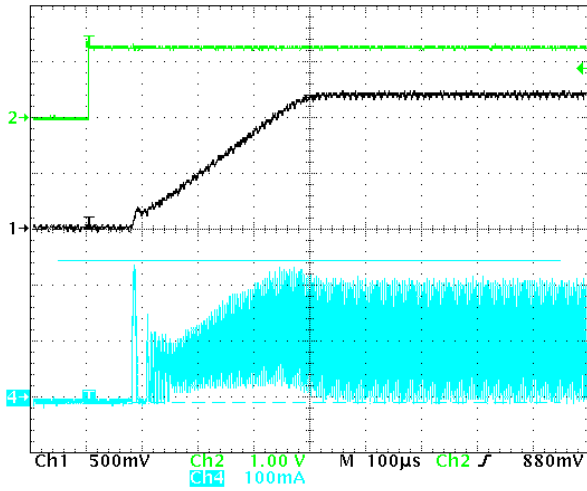
Figure 21. Typical Soft-Start ( V_{IN} = 3.6\text{ V} , V_{OUT} = 1.2\text{ V} , I_{OUT} = 100\text{ mA} , Temperature = 25°C)
