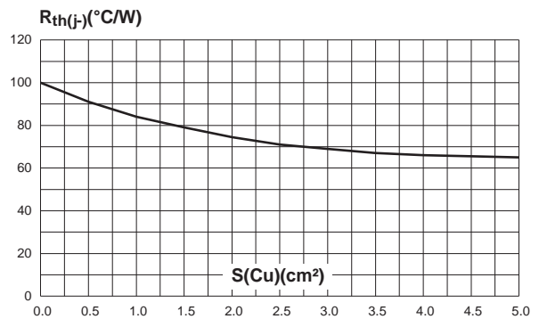
Fig. 8: Thermal resistance junction to ambient versus copper surface under each lead (Epoxy printed circuit board FR4, Cu: 35µm) (SMB).
