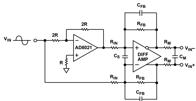
Figure 36. Single-Ended-to-Differential Conversion
