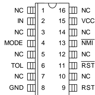
DS1231S 16-Pin SOIC (300-mil) See Mech. Drawings Section
