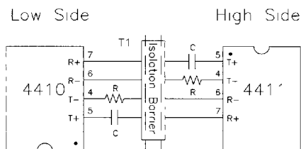
Fig. 10: Suggested IC Orientation
