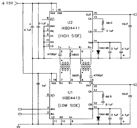
Fig. 1a: IXBD4410/4411 Switching time test circuit
