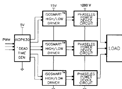
Fig. 8: Typical 3-phase motor control system block diagram
