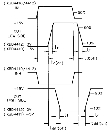
Fig. 1c: Output signal waveform
