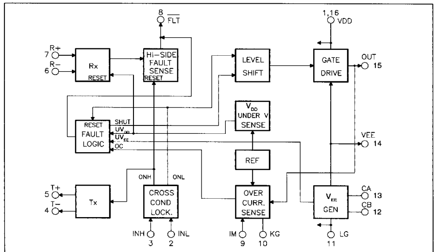
Fig. 3: IXBD4410, low-side driver block diagram
