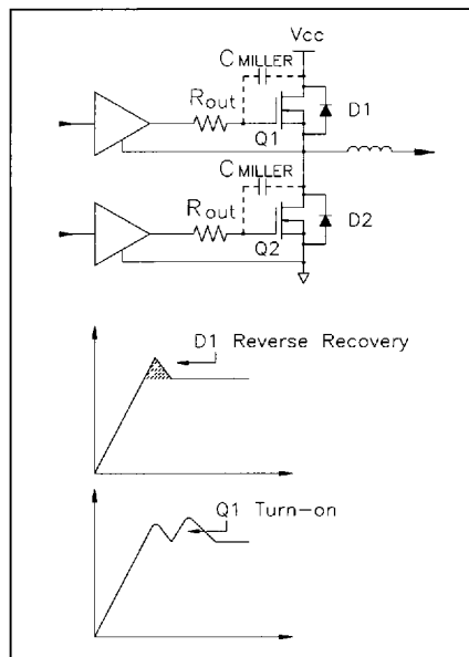
Fig. 5: Switching a clamped inductive load
