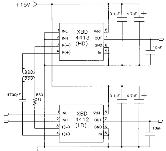
Figure 1b: IXBD4412/4413 Switching time test circuit
