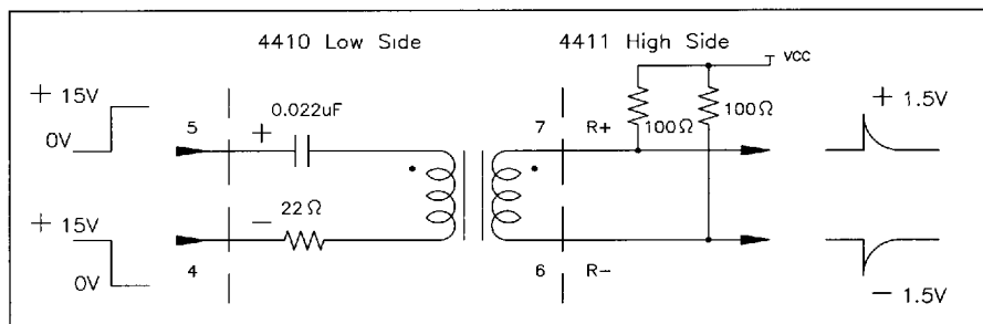
Fig. 13: Transmitter/Receiver Waveforms
