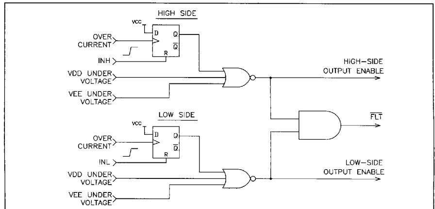
Fig. 4: Logic representation of IXBD4410 FLT signal
