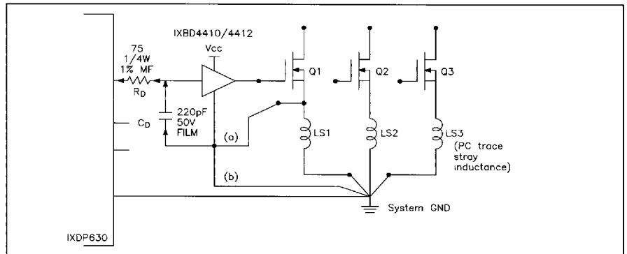
Fig. 11: Potential layout problems that create functional problems
