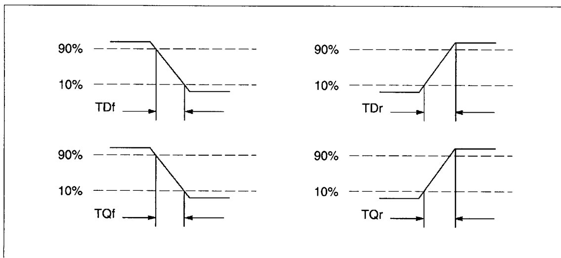
Figure 8.3 IMS T400 input and output edge timing
