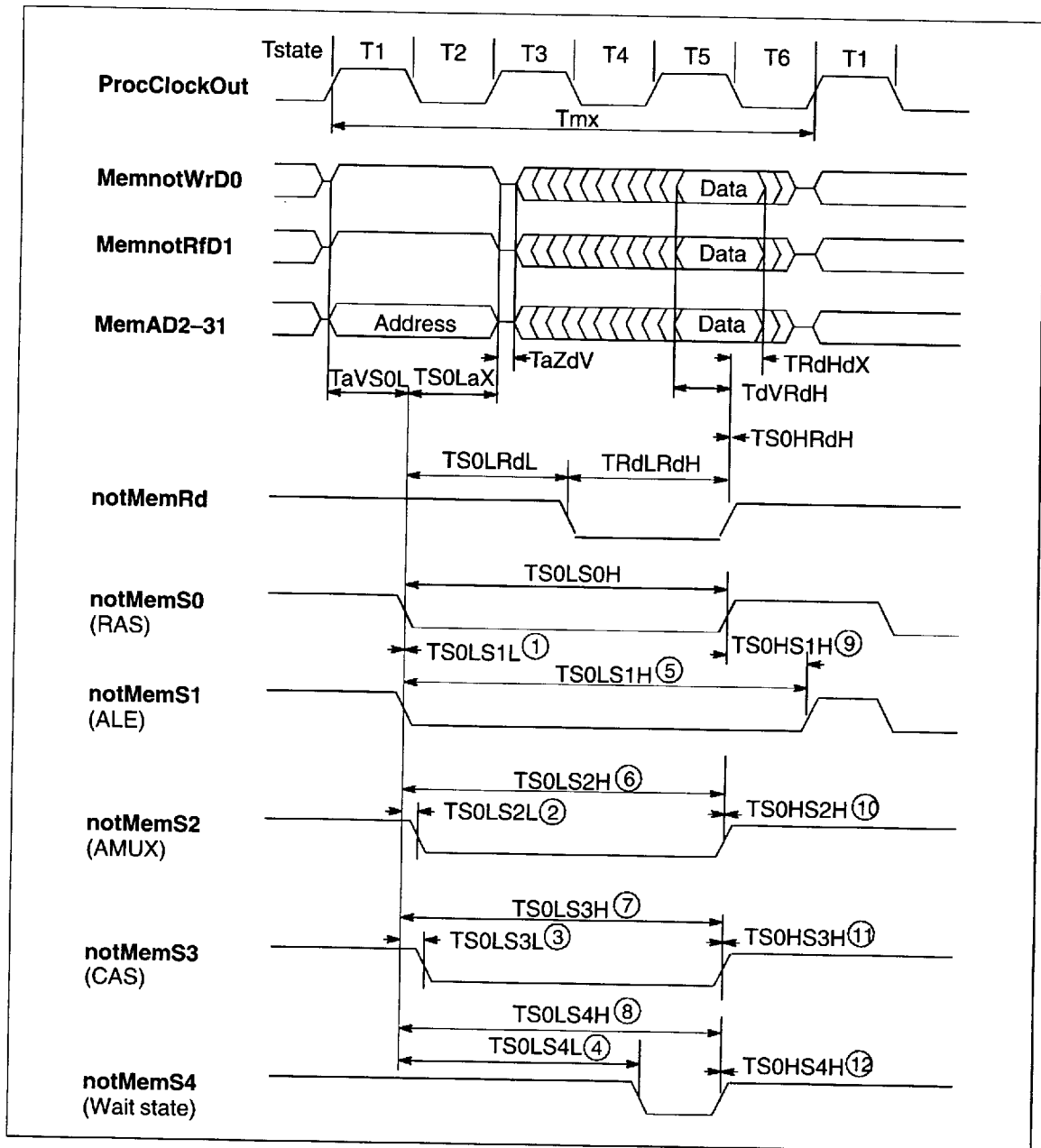
Figure 5.5 IMS T400 external read cycle: dynamic memory
