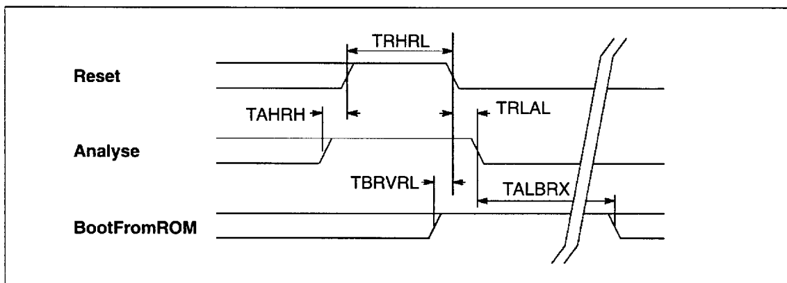
Figure 3.5 Transputer Reset , Analyse and BootFromROM timing
