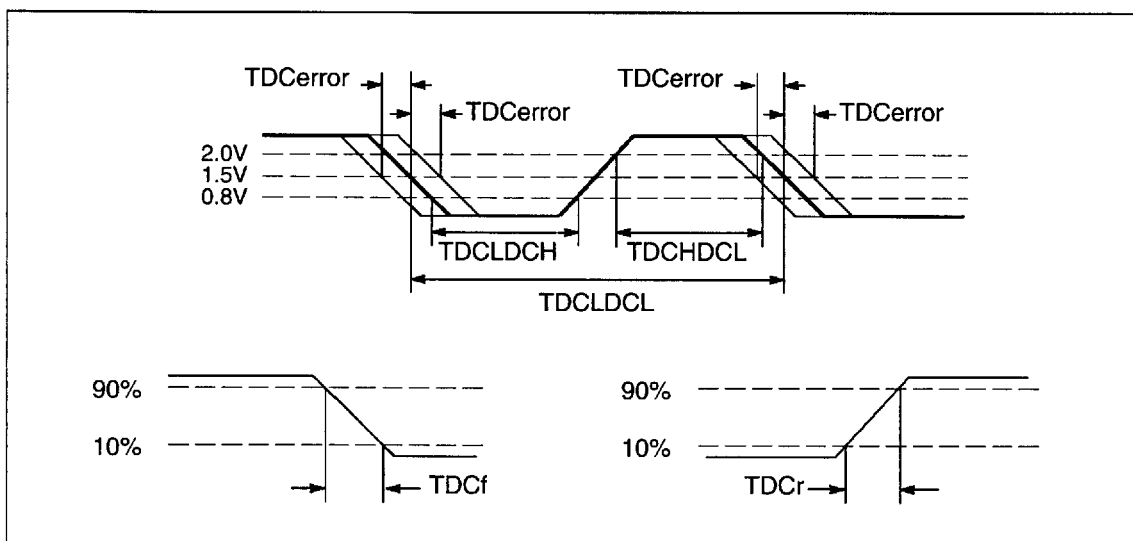
Figure 3.2 ClockIn timing
