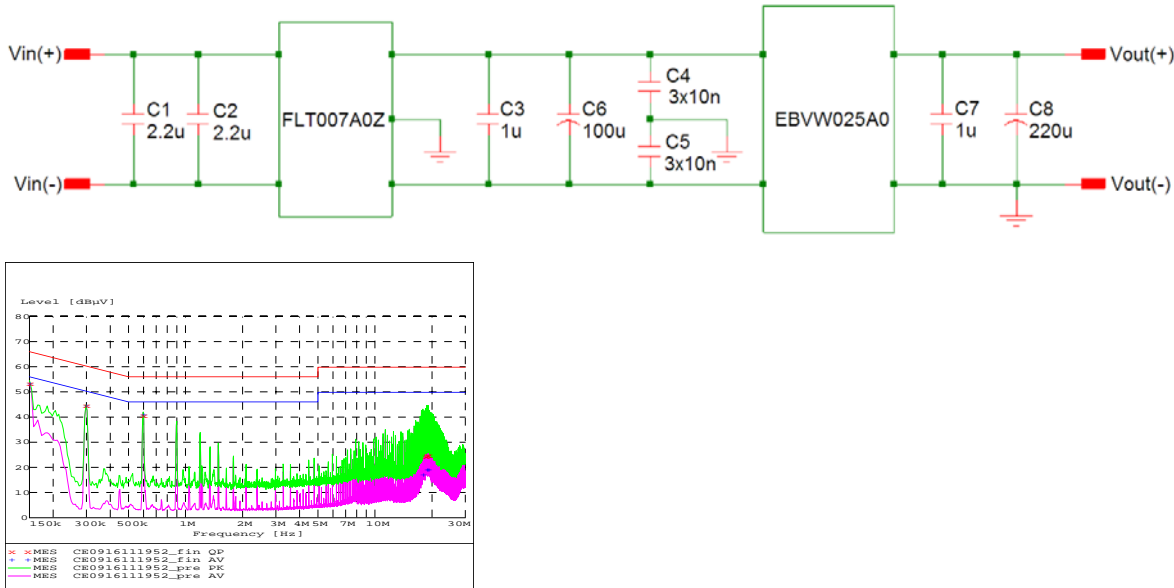
Figure 24. EMC Considerations.
