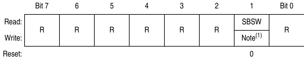
Figure 17-6. Break Status Register (BSR)
