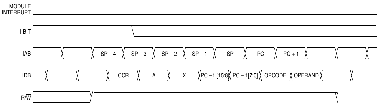
Figure 8-10. Interrupt Recovery
