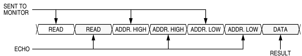
Figure 10-5. Read Transaction
