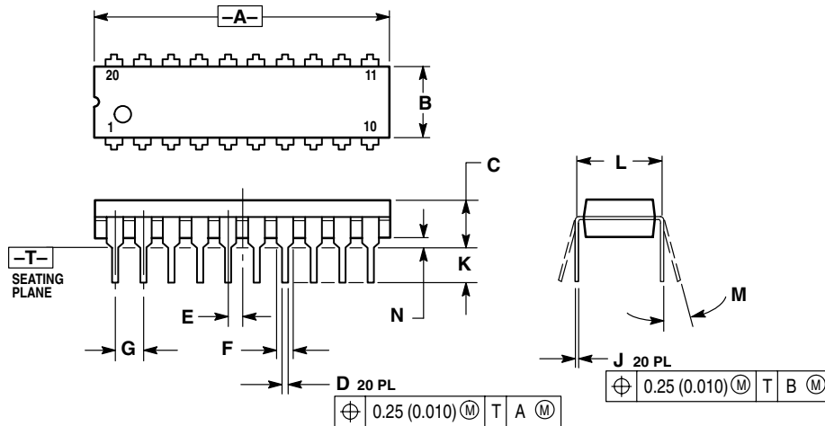
Figure 19-3. 20-Pin PDIP (Case 738)
