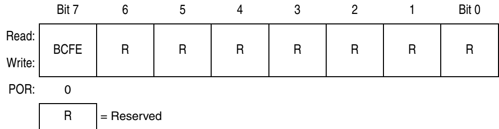
Figure 8-20. Break Flag Control Register (BFCR)
