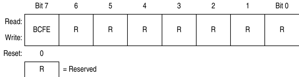
Figure 17-7. Break Flag Control Register High (BFCR)
