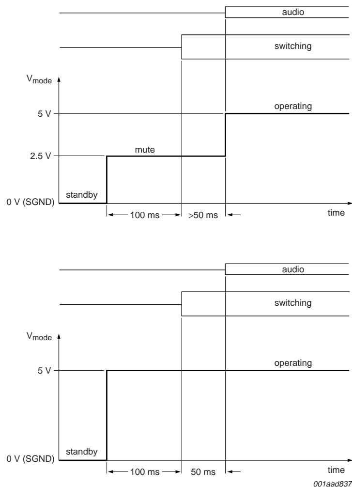
Fig 4. Timing on mode selection input
