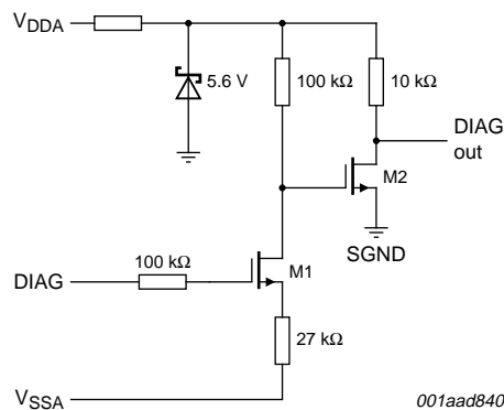
Fig 7. DIAG readout circuit with level shift
