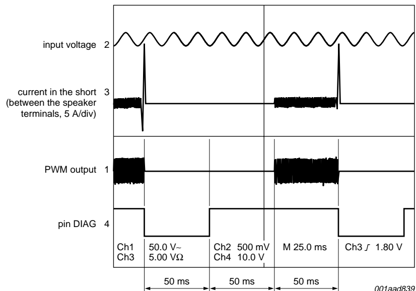
Fig 6. Restart of the TDF8590TH
