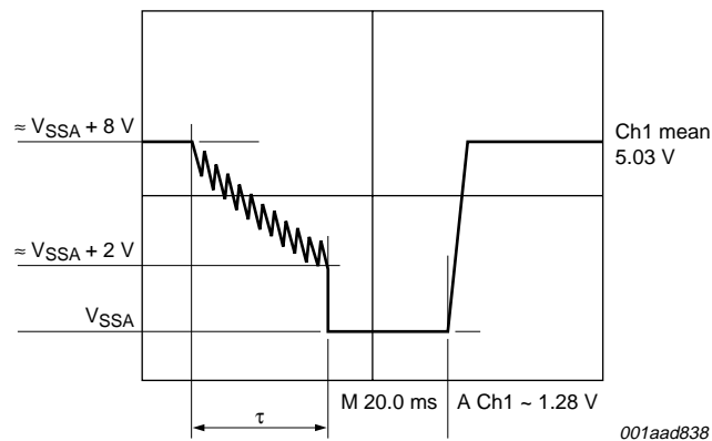
Fig 5. Pin DIAG with activated current limiting
