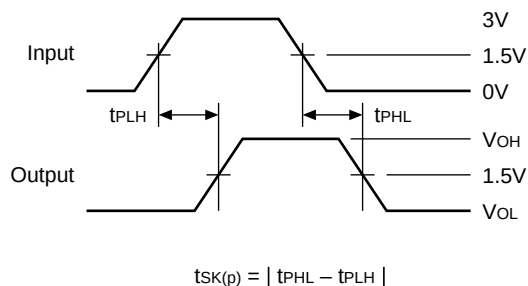
Pulse Skew – t_{SK(P)}
