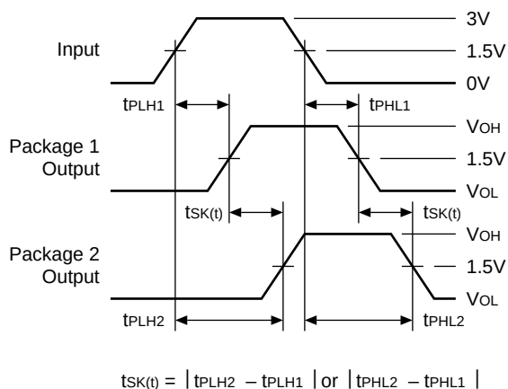
Package Skew – t_{SK(T)}
