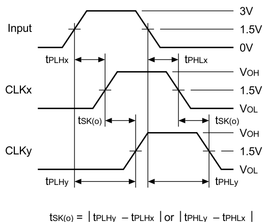
Output Skew – t_{SK(O)}
