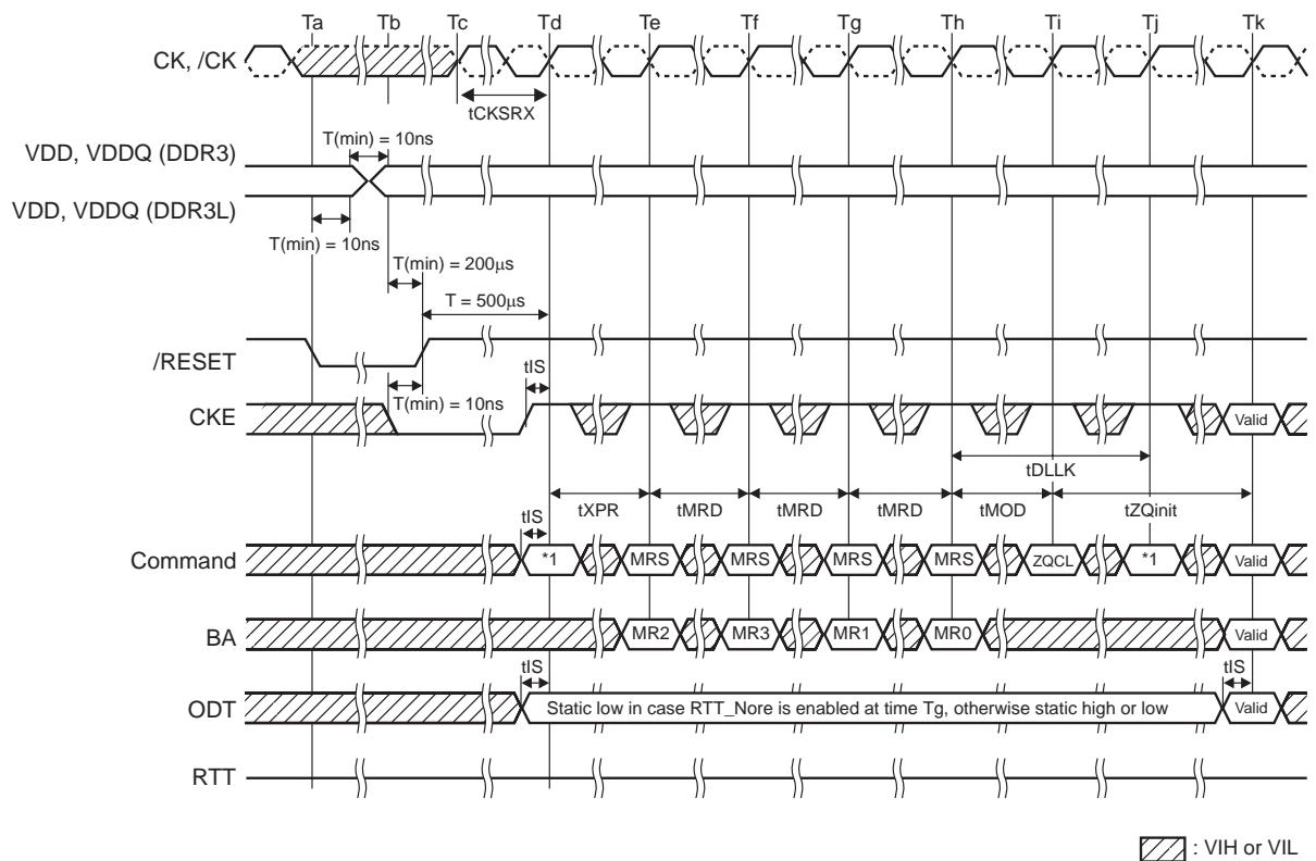
Figure 1: VDD/VDDQ Voltage Switch between DDR3L and DDR3
