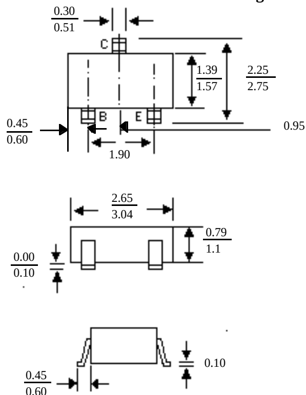
02 Package: SOT-23J
