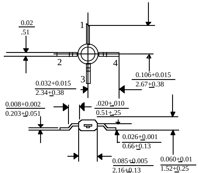
87 Package: 0.085" Plastic, Short Lead
