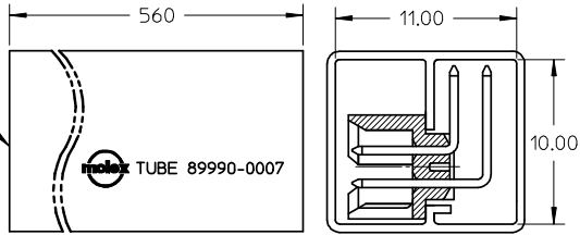
REF: ORIENTATION OF PART IN TUBE.
