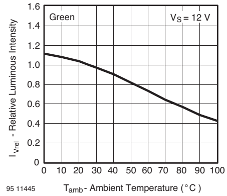
Figure 23. Rel. Luminous Intensity vs. Ambient Temperature
