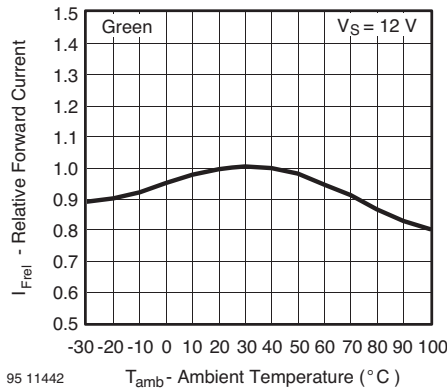
Figure 20. Relative Forward Current vs. Ambient Temperature
