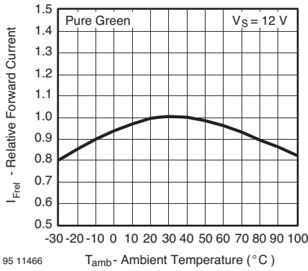
Figure 26. Relative Forward Current vs. Ambient Temperature
