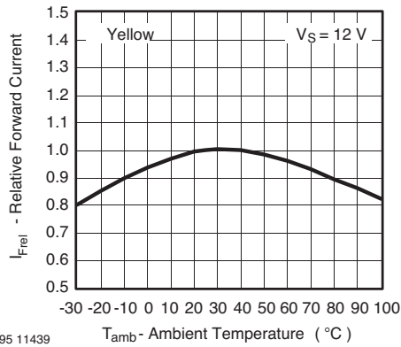
Figure 14. Relative Forward Current vs. Ambient Temperature
