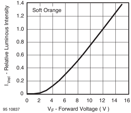
Figure 10. Relative Luminous Intensity vs. Forward Voltage
