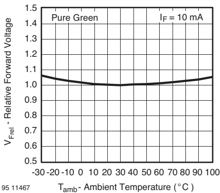
Figure 27. Relative Forward Voltage vs. Ambient Temperature
