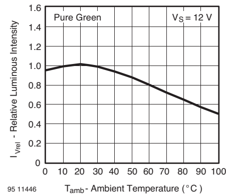
Figure 29. Rel. Luminous Intensity vs. Ambient Temperature
