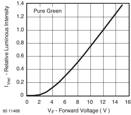
Figure 28. Relative Luminous Intensity vs. Forward Voltage
