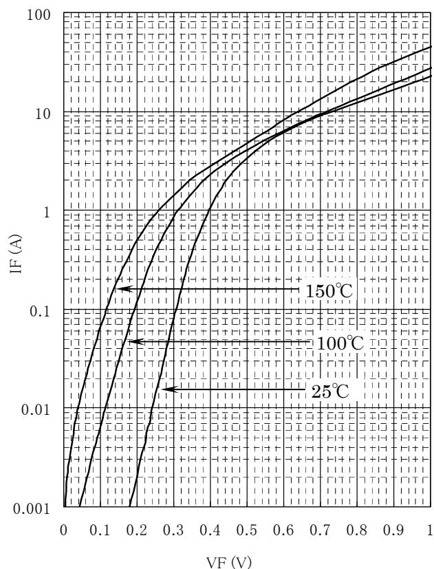
SJPB-L4 IF-VF Characteristics
