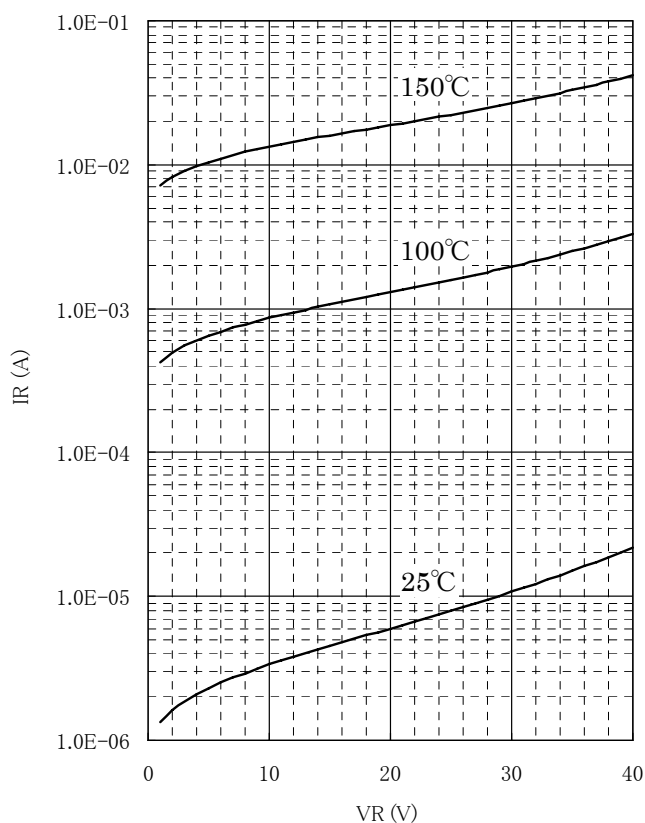
SJPB-L4 VR-IR Characteristics
