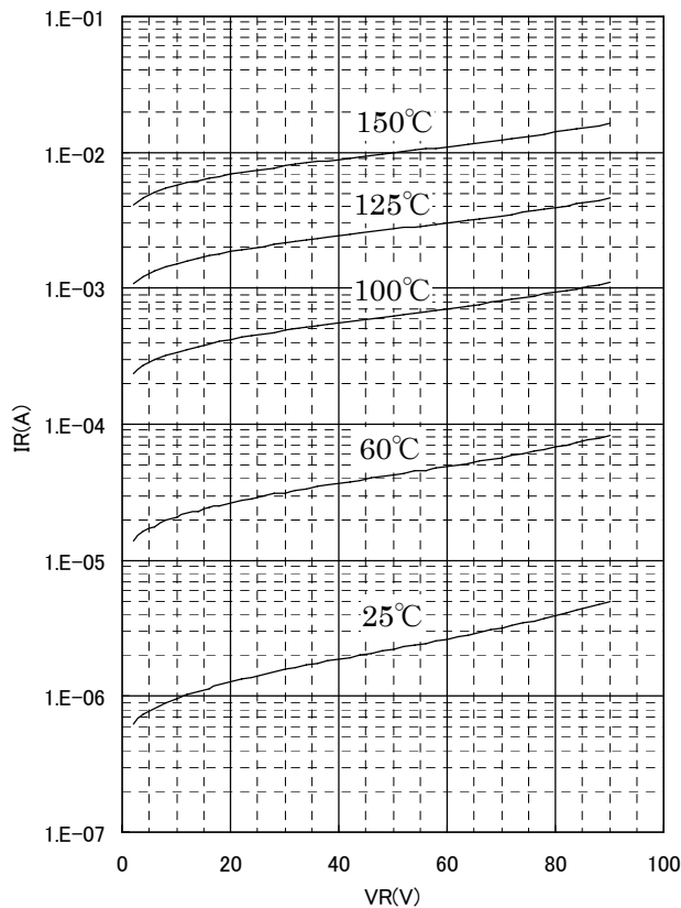
SJPB-H9 VR-IR Characteristics
