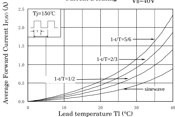
Current Derating
