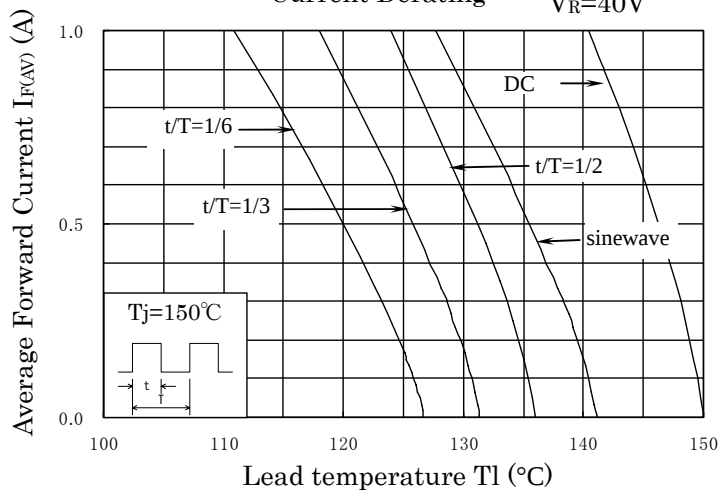
Current Derating
