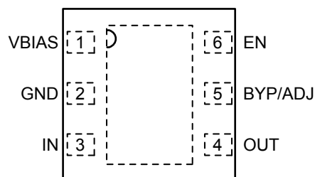
6-Pin 2mm x 2mm Thin MLF ® (MT)
