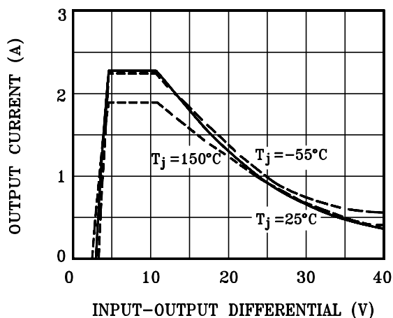
Current Limit
