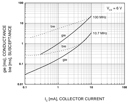
Figure 7. yie - f
