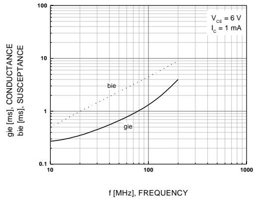
Figure 18. yie - f
