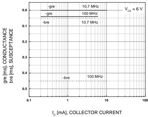
Figure 9. yre - f
