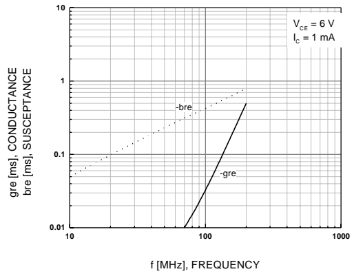
Figure 14. yre - f
