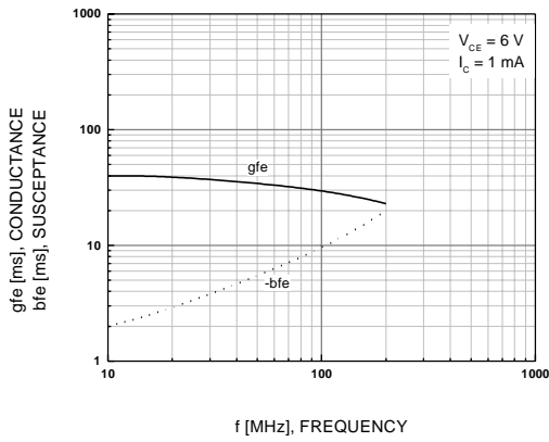
Figure 15. yfe - f
