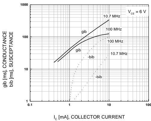
Figure 11. yib - f
