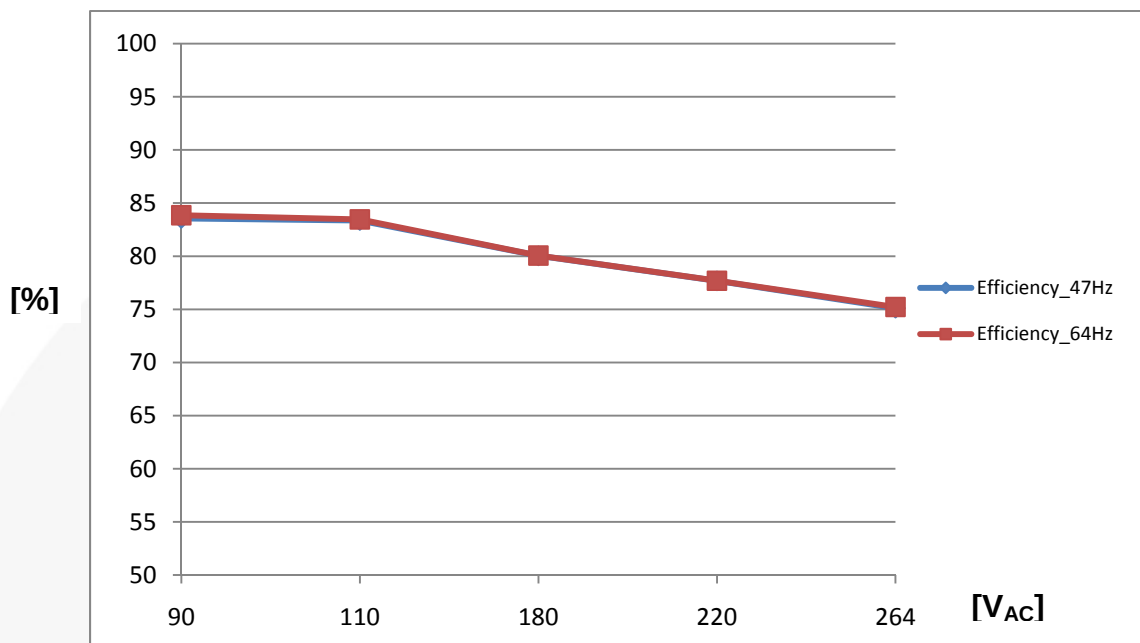
Figure 28. System Efficiency
