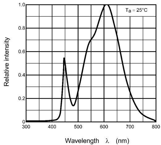
Fig. 8.4 Wavelength characteristic
