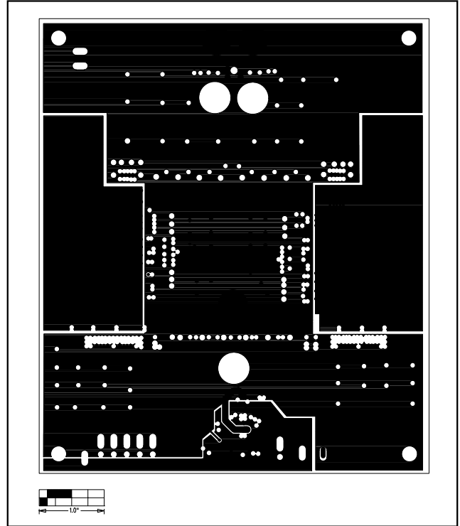
Figure 5. MAX1938 EV Kit PC Board Layout—Inner Layer 3
