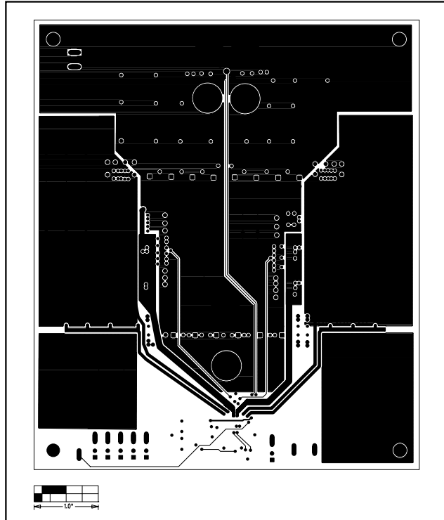
Figure 6. MAX1938 EV Kit PC Board Layout—Solder Side
