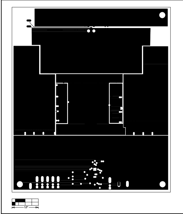
Figure 4. MAX1938 EV Kit PC Board Layout—Inner Layer 2
