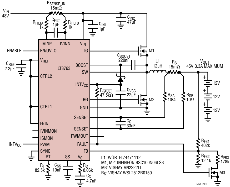
36V SLA Battery Charging
