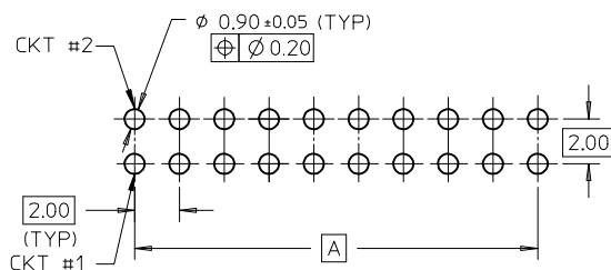
RECOMMENDED PCB PATTERN
