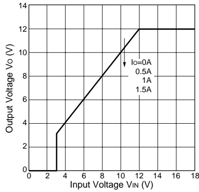
Output Voltage(SI-3121N)
