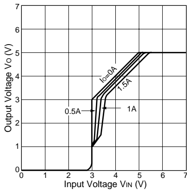
Output Voltage(SI-3051N)
