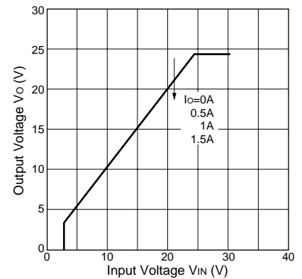
Output Voltage(SI-3241N)
