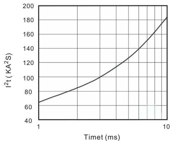
Fig.6 I^2t Characteristic
