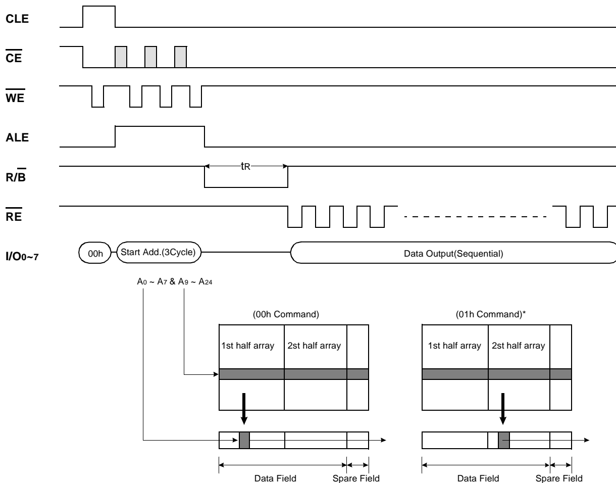
Figure 3. Read1 Operation
