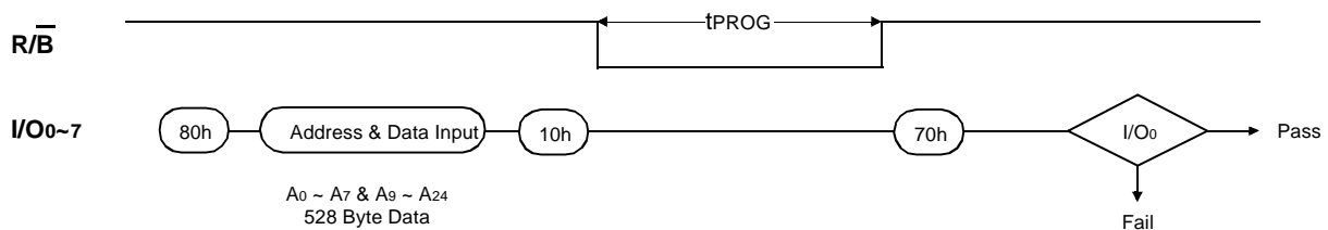
Figure 7. Program Operation
