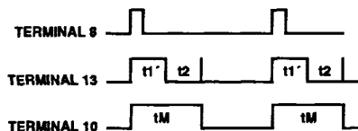
FIGURE 30. MONOSTABLE WAVEFORMS
