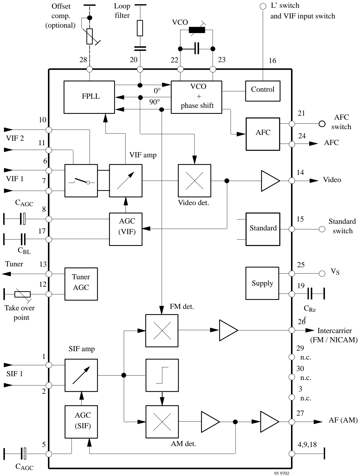
Figure 1. Block diagram
