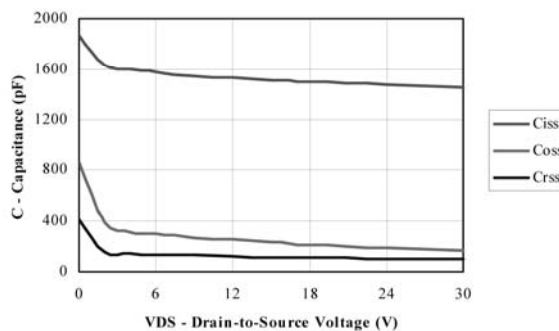
Capacitance
