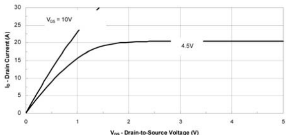
Output Characteristics
