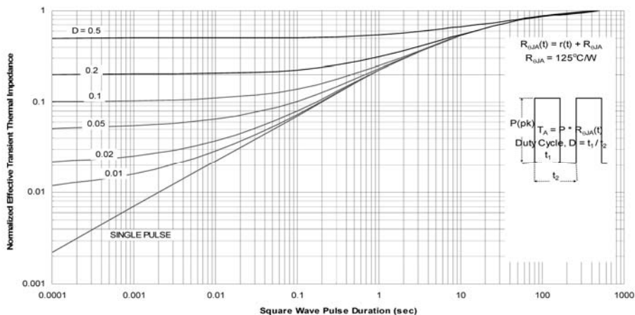
Normalized Thermal Transient Impedance, Junction-to-Ambient
