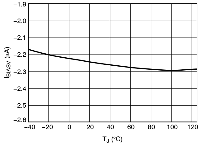
Figure 13. IBIASV at V CC = 15 V, V SNS > V SNSBIASLH
