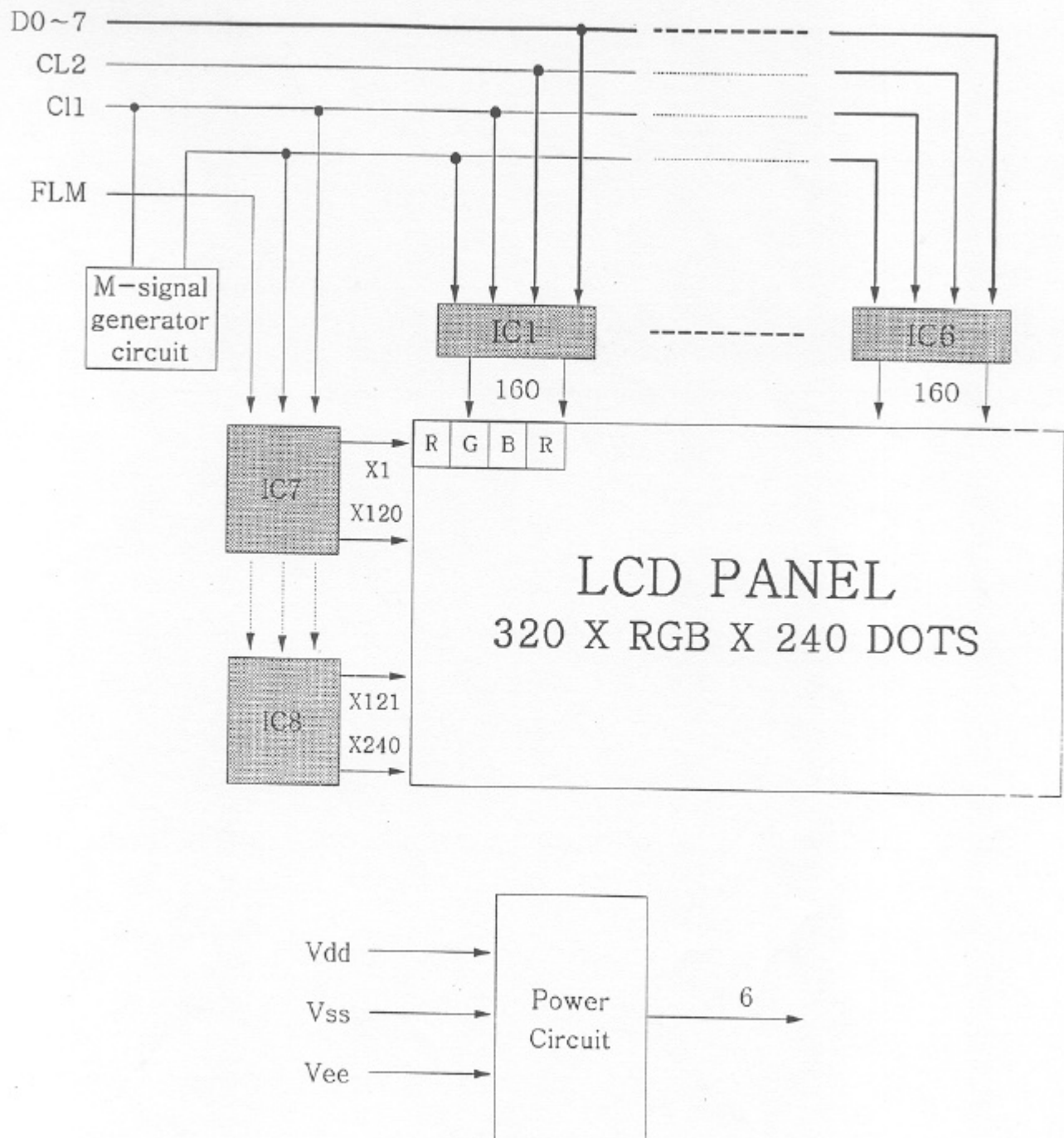
Fig. 8-1 Block diagram
