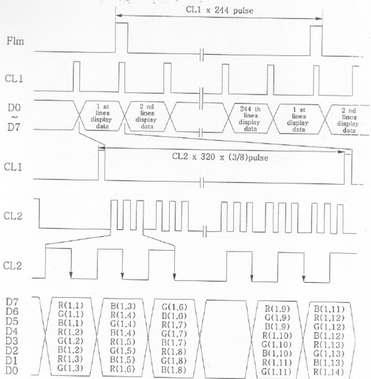
Fig. 8-3 Signal timing (2)
