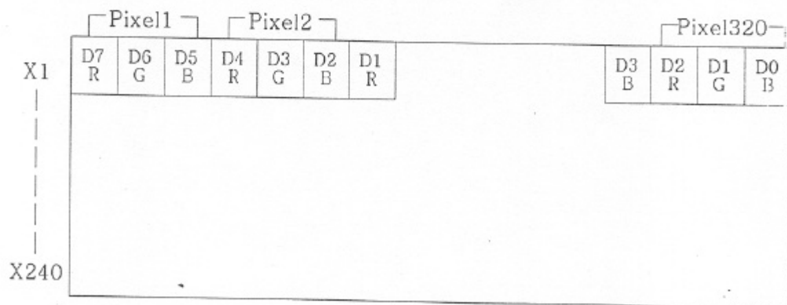
Fig. 8-3 Signal timing (2)
