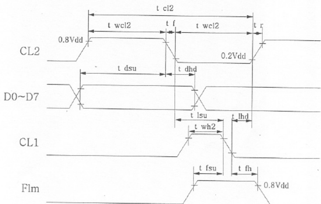
Fig. 8-2 Signal timing (1)
