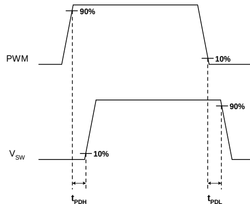
Figure 10 Timing Diagram
