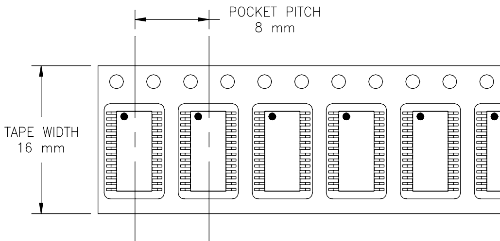
Figure 17: Tape Dimensions
