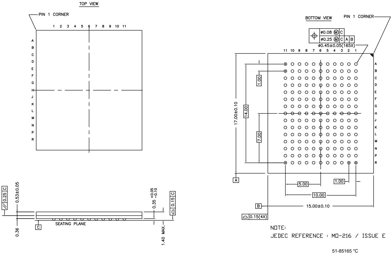
Figure 8. 165-ball FBGA (15 x 17 x 1.4 mm)
